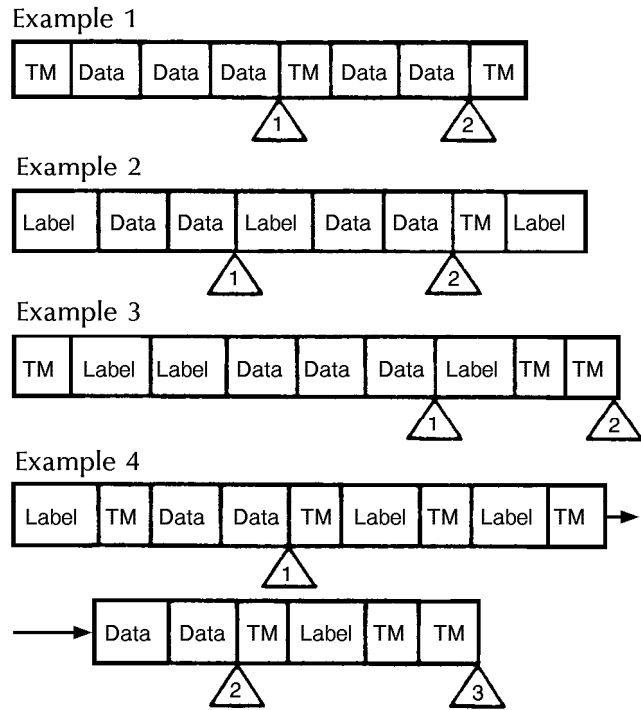
Figure 14-1. Undefined labeled tape structures
