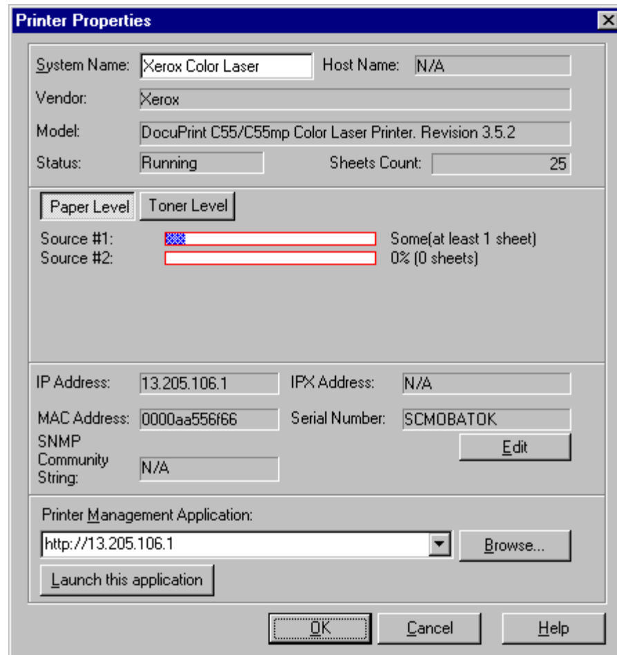
Figure 27 Printer Properties window
