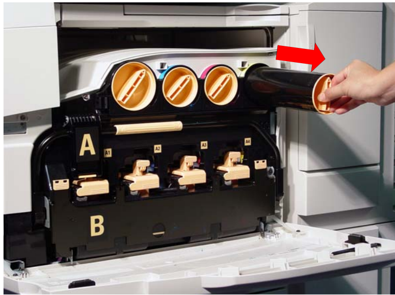
Fig. 3 Gently pull the toner cartridge towards you to remove.
