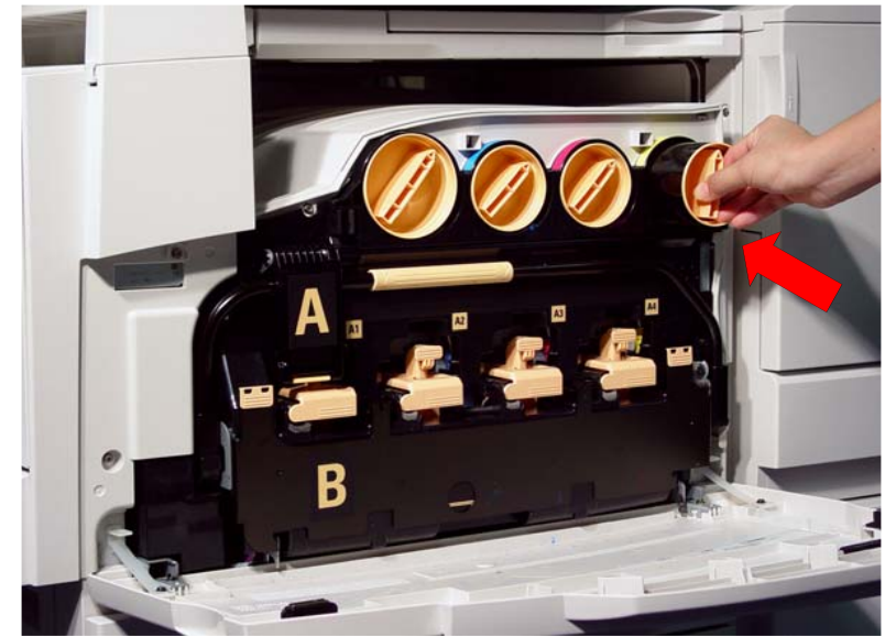
Fig. 5 Insert the toner cartridge as far as possible with the arrow on the cartridge facing up.
