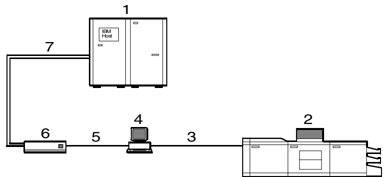
Figure 1-1. Xerox 4050/4090 IPS: channel-attached configuration
