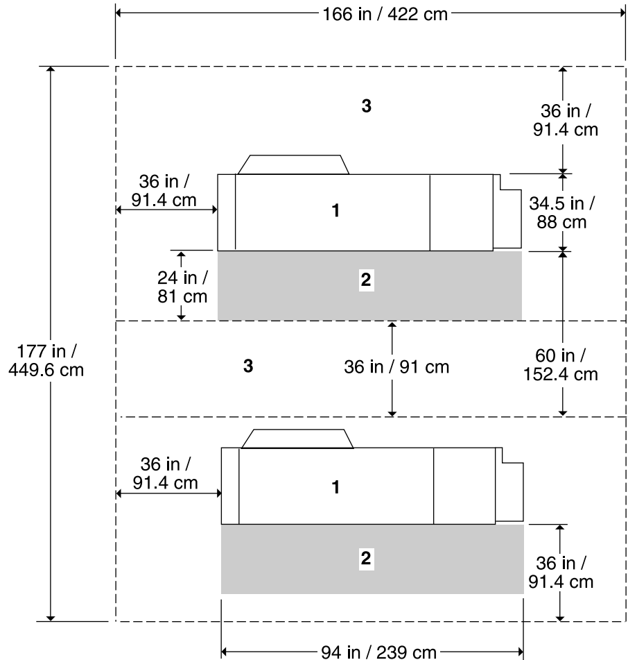
Figure 6-8. Face-to-back shared service area space
