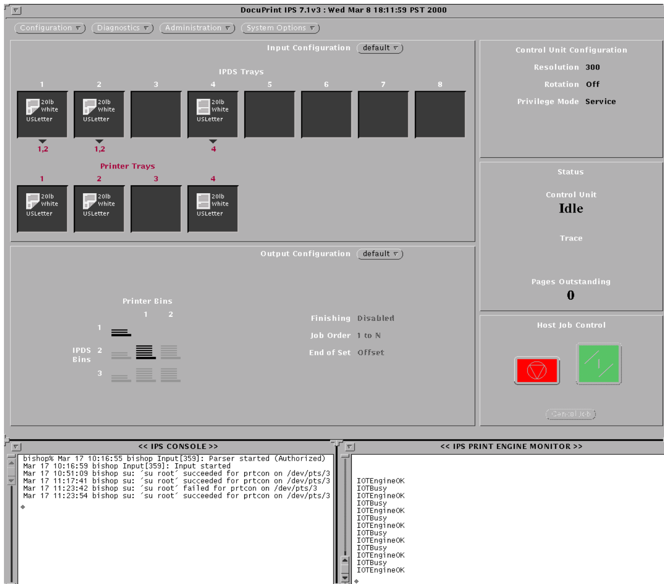
Figure 2-6. IPS user interface screen
