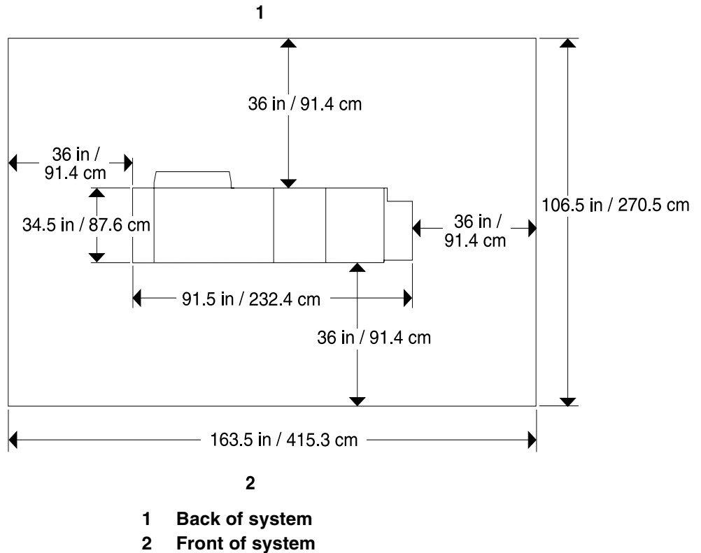
Figure 6-2. 4050/4090 printer with dual stacker
