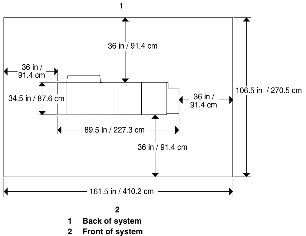
Figure 6-3. 4050/4090 printer with stitcher/stacker
