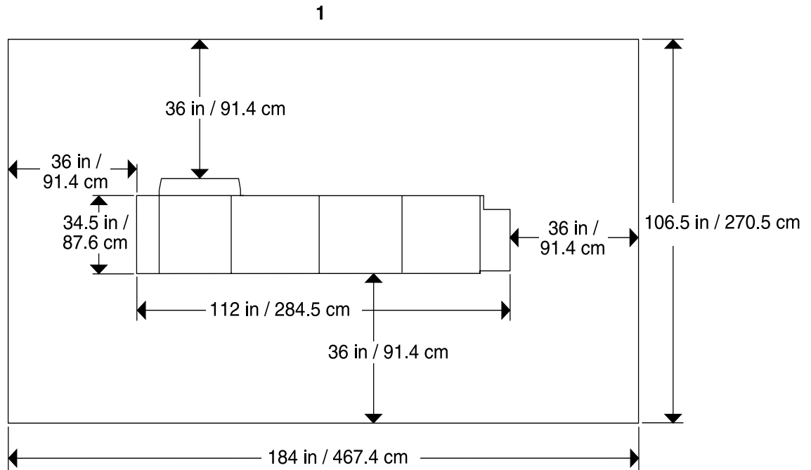
Figure 6-5. 4050/4090 printer with high-capacity feeder and stitcher/stacker
