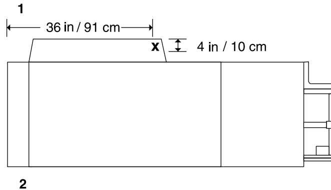
Figure 7-1. 4050/4090 cable enter/exit location (top view)
