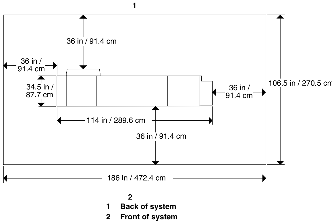
Figure 6-4. 4050/4090 printer with high-capacity feeder and dual stacker
