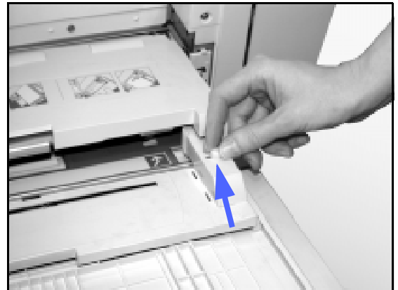
Figure 119: Front Paper Guide and registration thumb screw
