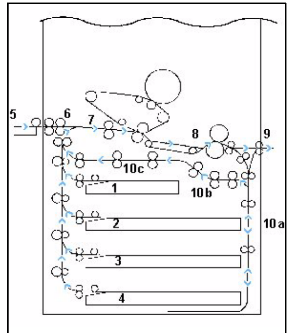
Figure 16: Paper Path
