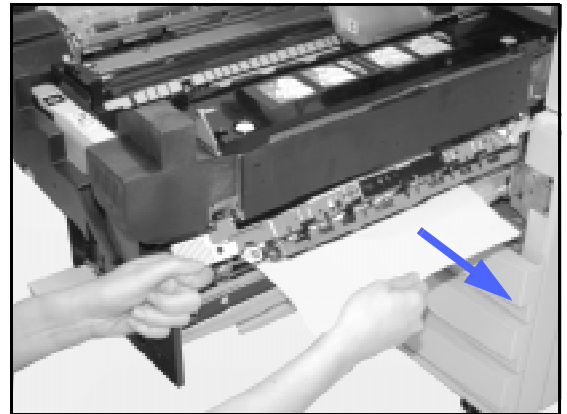
Figure 12: Fuser Exit area
