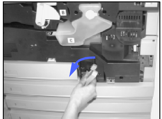
Figure 14: Rotating the green handle anti-clockwise
