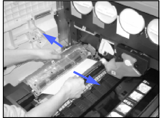
Figure 10: Area 1 in the Registration area
