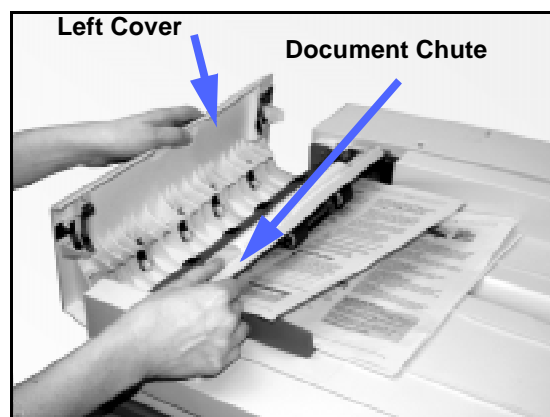
Figure 125: Opening the Left Cover and the Document Chute
